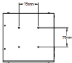
STANDARD MOUNTING PATTERN FOR USE WITH AM SCREWS
